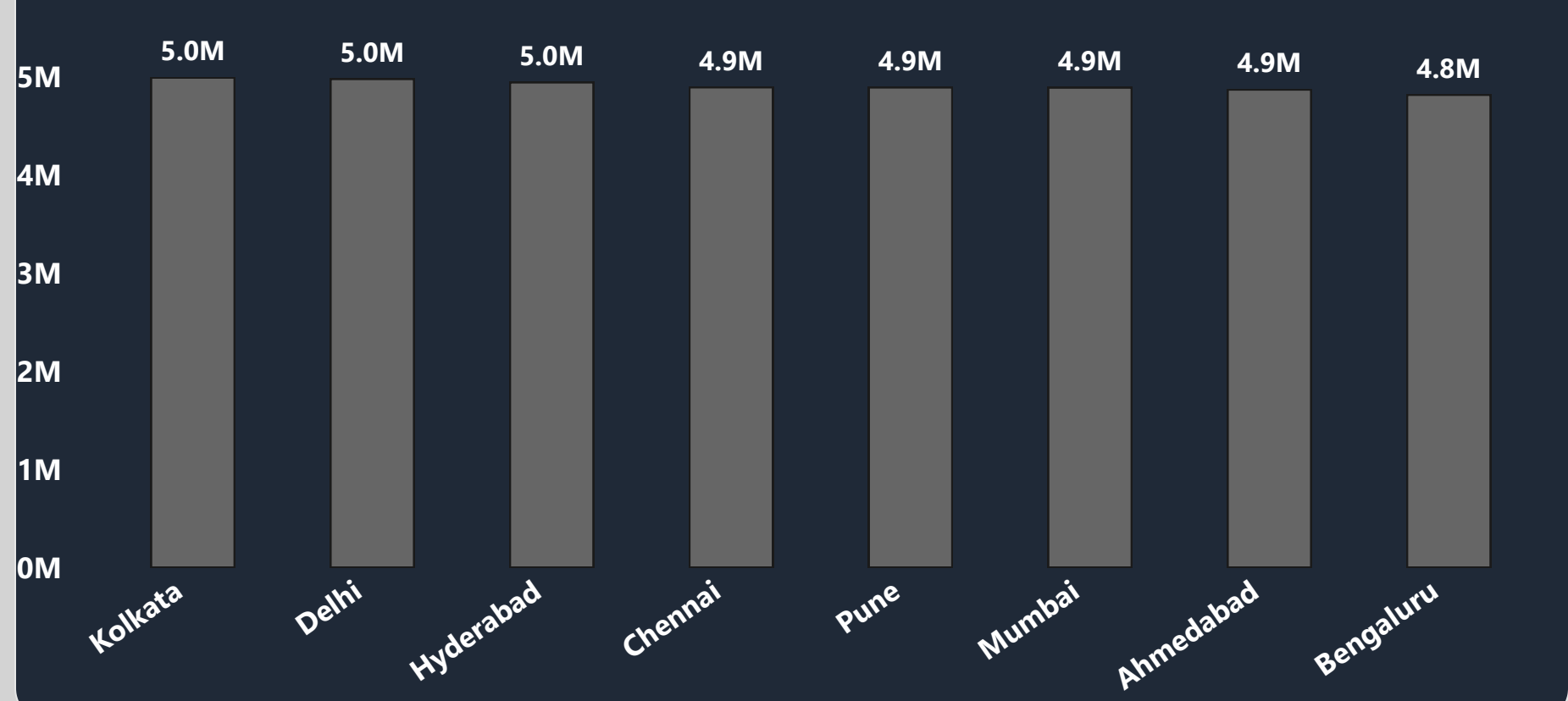
City Performance
